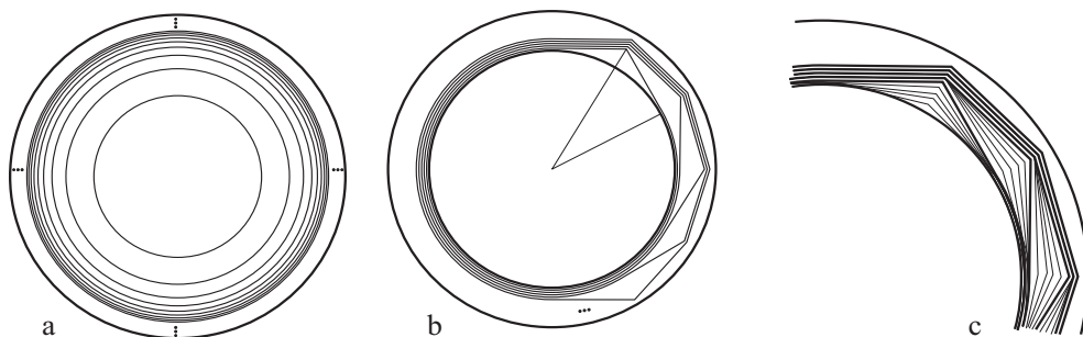
Fig. 5. A \Subset -nested arc with infinite length
