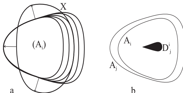
Fig. 3. Counterexample showing that additivity is not sufficient
