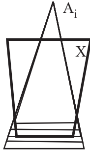
Fig. 11. A non-Čebyšev family of homothets
