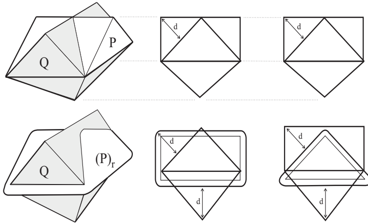
Fig. 12. A family of parallel bodies with non-Čebyšev translates
