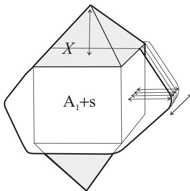
Fig. 6. Strict convexity is necessary in more than two dimensions.
