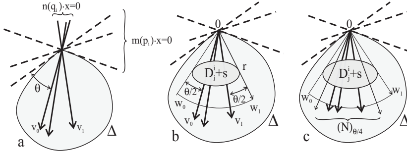
Fig. 8. The case in which every line of N^\perp intersects \text{int } \Delta
