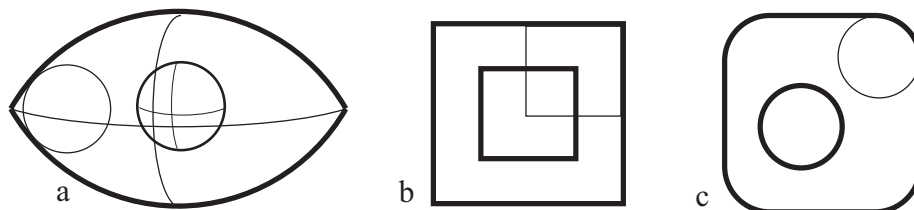
Fig. 4. Examples illustrating non-implications among containment properties
