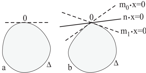
Fig. 10. The case in which some line of N^\perp does not intersect \text{int } \Delta
