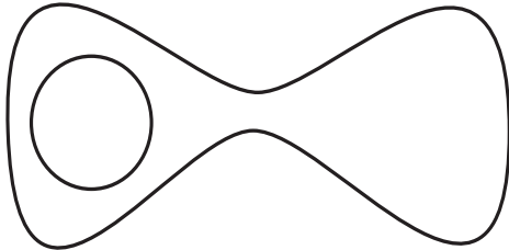
Fig. 1. The smaller body cannot be centered within the larger one.
