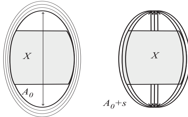
Fig. 7. A body equidistant from various translates of A_0
