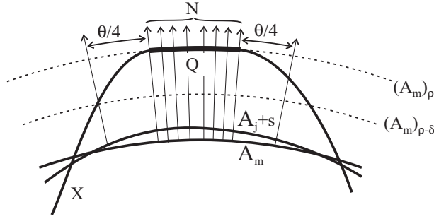
Fig. 9. The configuration near Q
