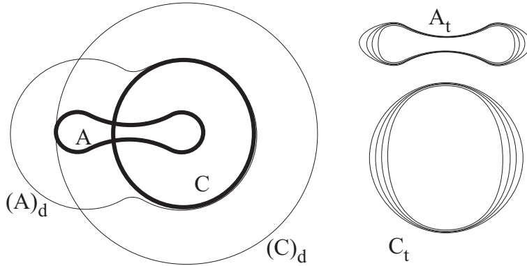
Fig. 2. Counterexample showing that convexity is essential
